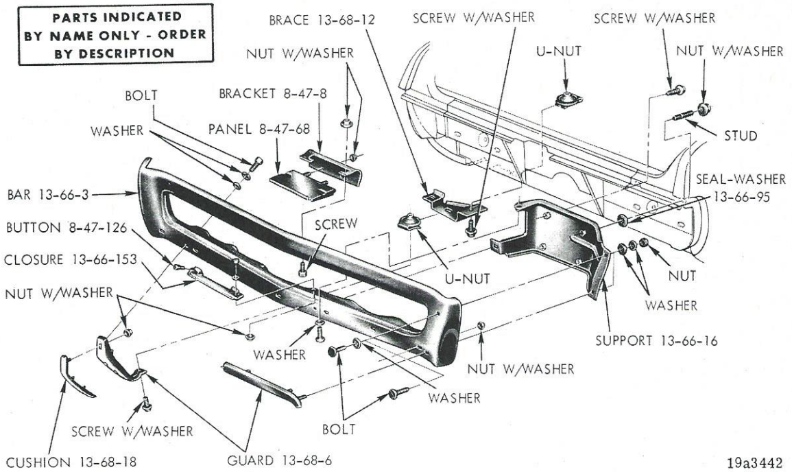
REAR BUMPER - CORONET 2 D., 2 D. H. T. AND FASTBACK
