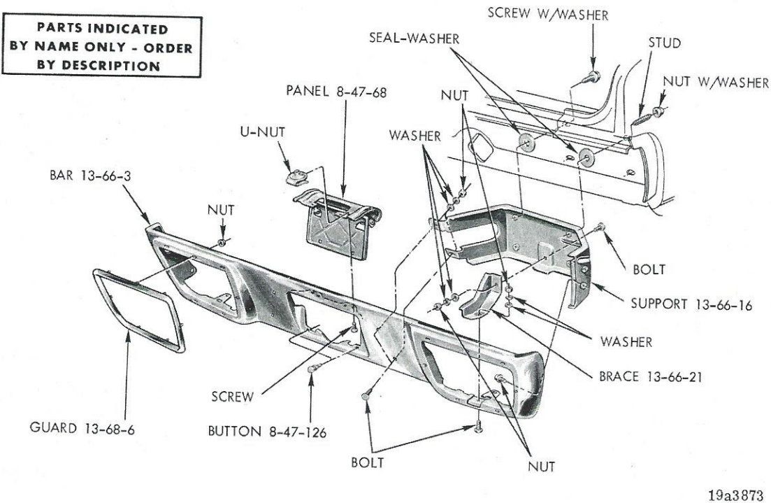
REAR BUMPER - SATELLITE 2 D. AND 2 D. H.T.
