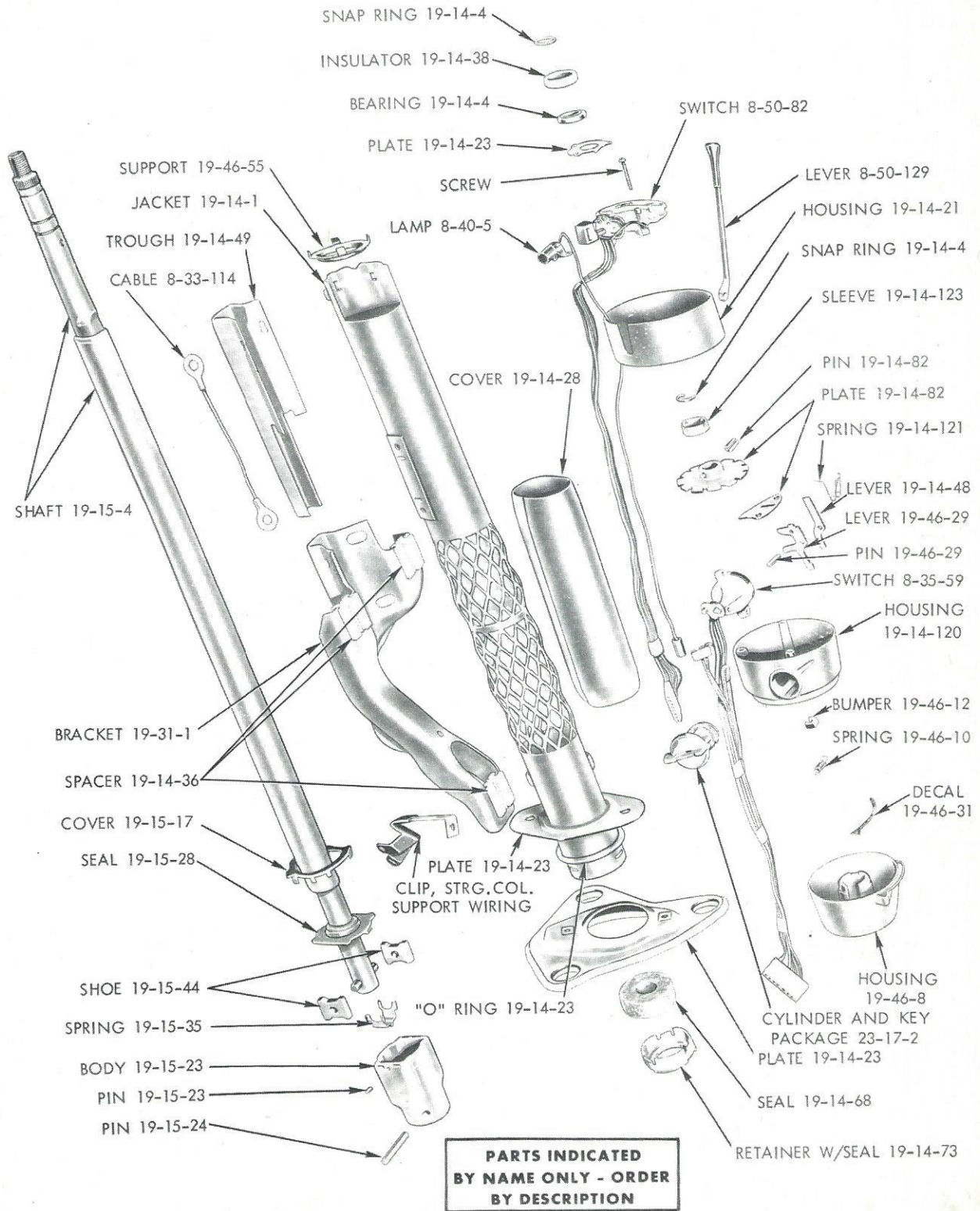
STEERING COLUMN ASSEMBLY - FLOOR SHIFT - (STANDARD AND AUTOMATIC TRANSMISSION)
