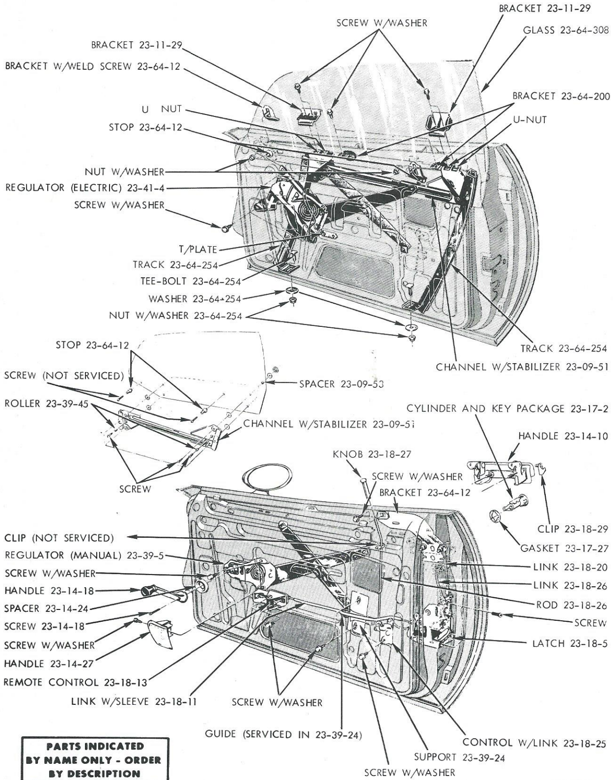
FRONT DOOR INSIDE PANEL - SATELLITE AND CORONET 2 DOOR SEDAN, 2 DOOR HARDTOP AND FASTBACK
