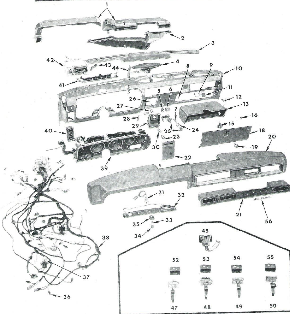
INSTRUMENT PANEL - SATELLITE, CORONET AND CHARGER
