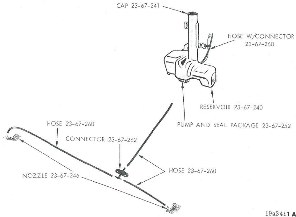
WINDSHIELD WASHER SYSTEM - SATELLITE, CORONET AND CHARGER
