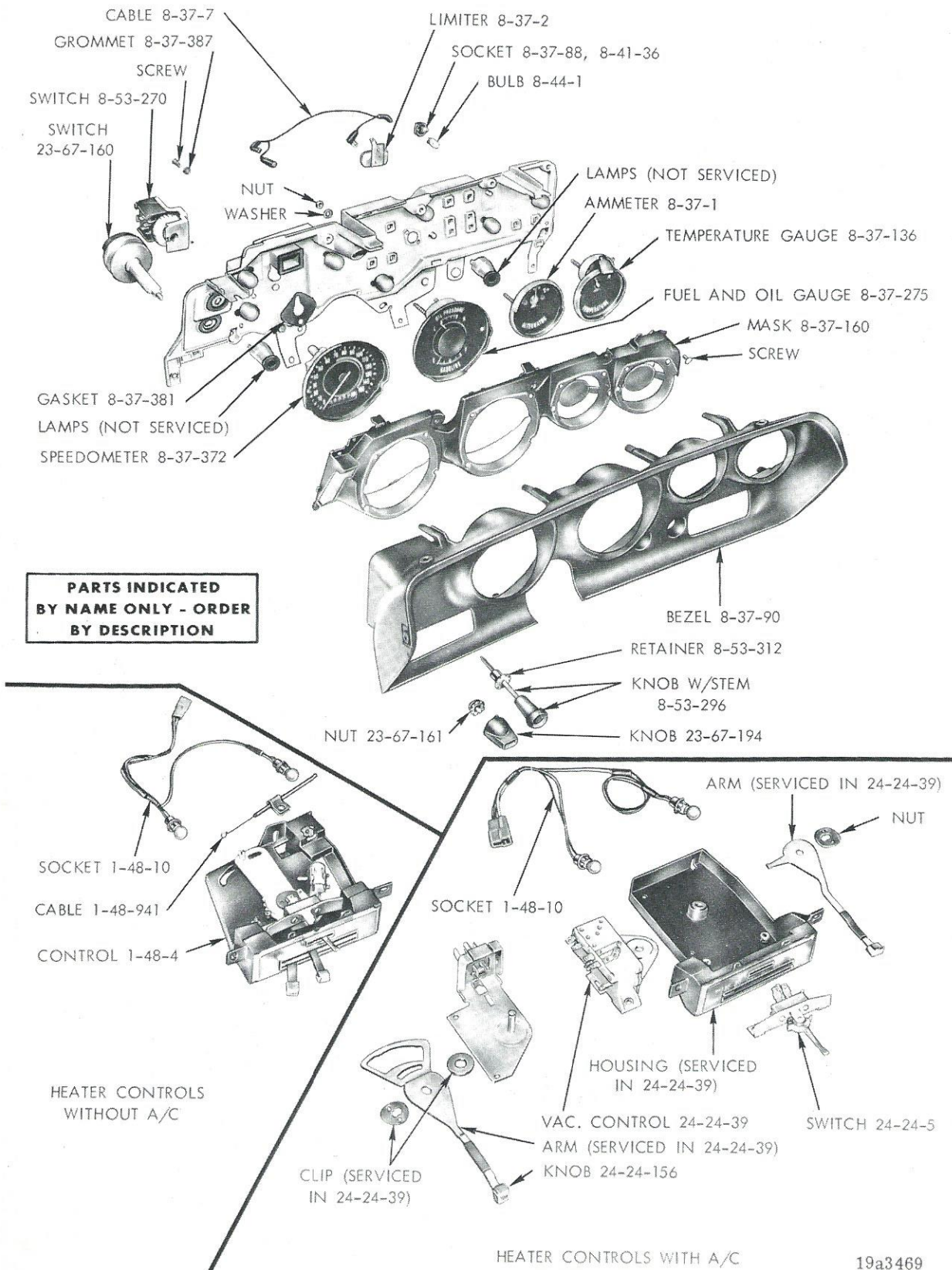
INSTRUMENT CLUSTER - R & W WITH RALLYE INSTRUMENT PANEL
