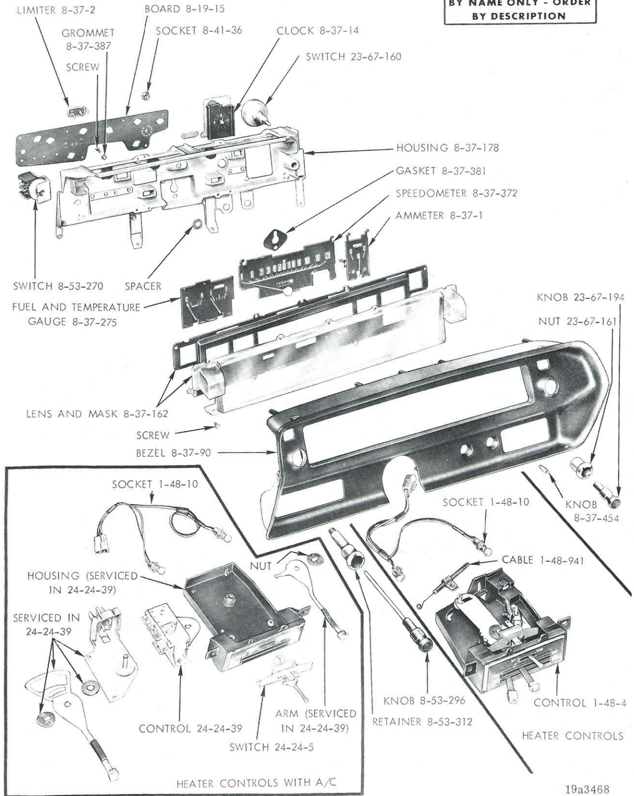
INSTRUMENT CLUSTER - R & W WITHOUT RALLYE INSTRUMENT PANEL
